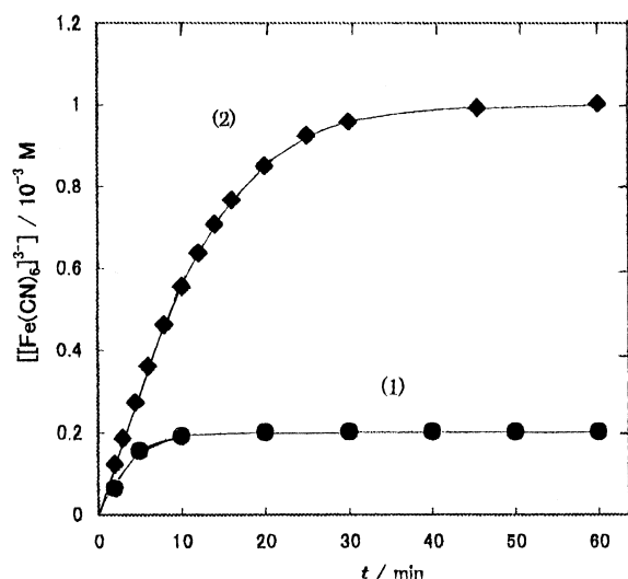
Fig. 6. Oxidation of [\text{Fe}(\text{CN})_6]^{4-} to [\text{Fe}(\text{CN})_6]^{3-} by PDP. Solution of 1.0 \times 10^{-3} M \text{K}_4[\text{Fe}(\text{CN})_6] was mixed with PDP of 1.0 \times 10^{-4} M and 1.0 \times 10^{-3} M in curves (1) and (2) under conditions of pH 4.05 and 25^\circ\text{C} , respectively.
