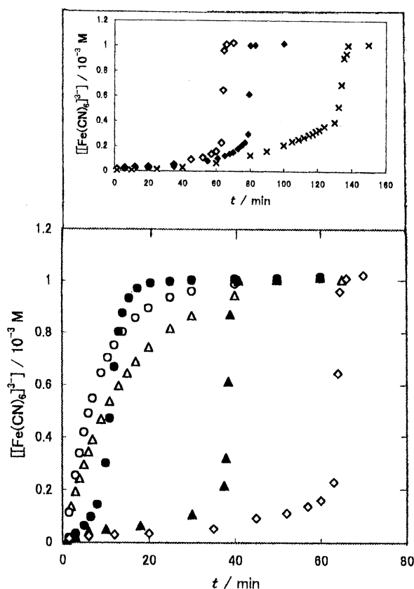
Fig. 7. Effect of phosphinate concentrations.
