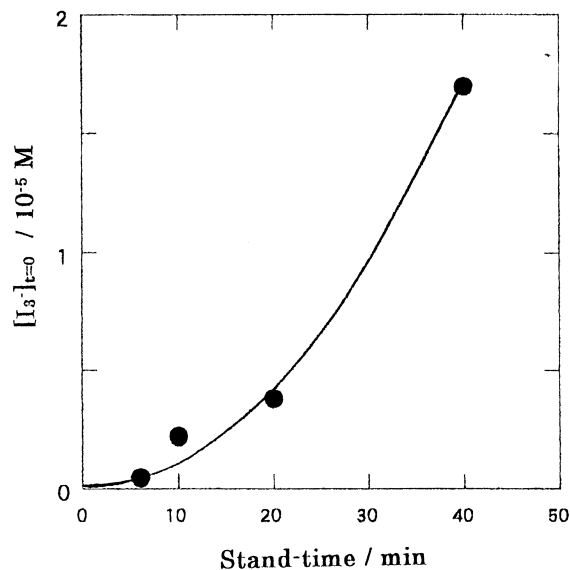
Fig. 2. Dependence of the standing time (stand-time) for the phosphinate solution on the formation of \text{I}_3^- .
