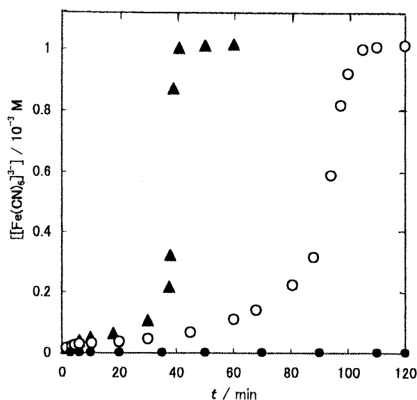
Fig. 3. Effect of the oxygen concentration.
