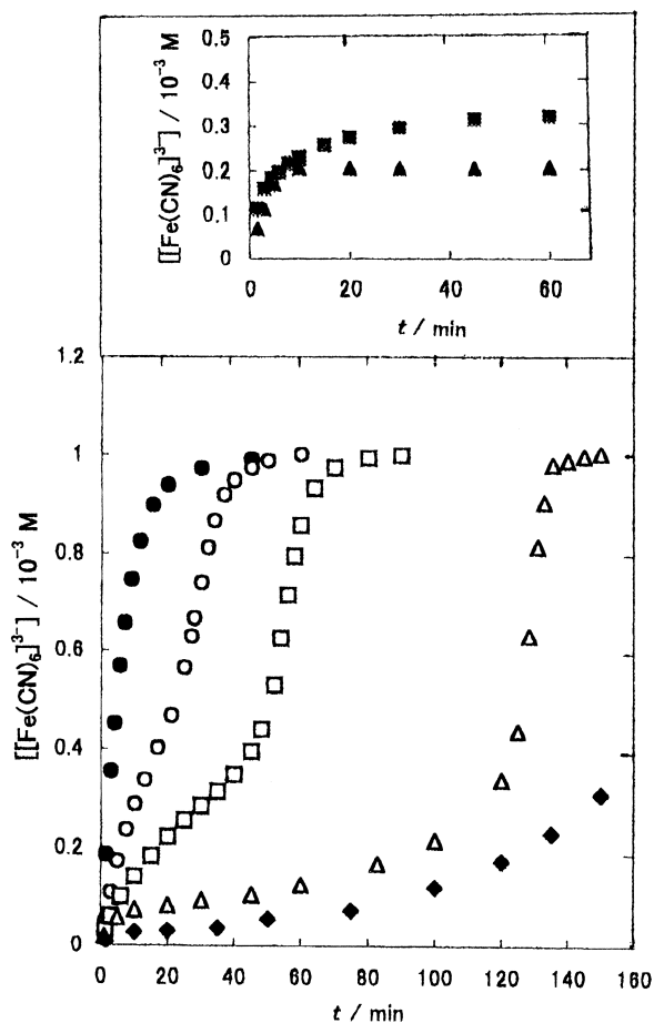
Fig. 5. Effect of PDP.
