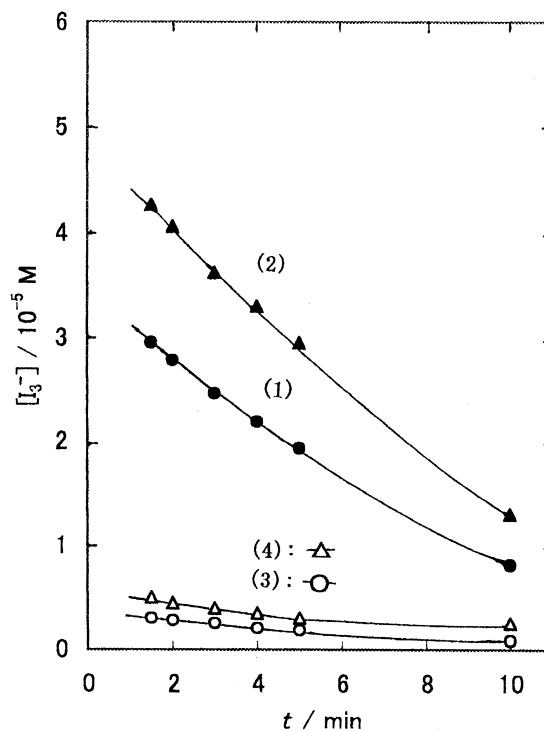
Fig. 1. Plots of [\text{I}_3^-] vs t .
