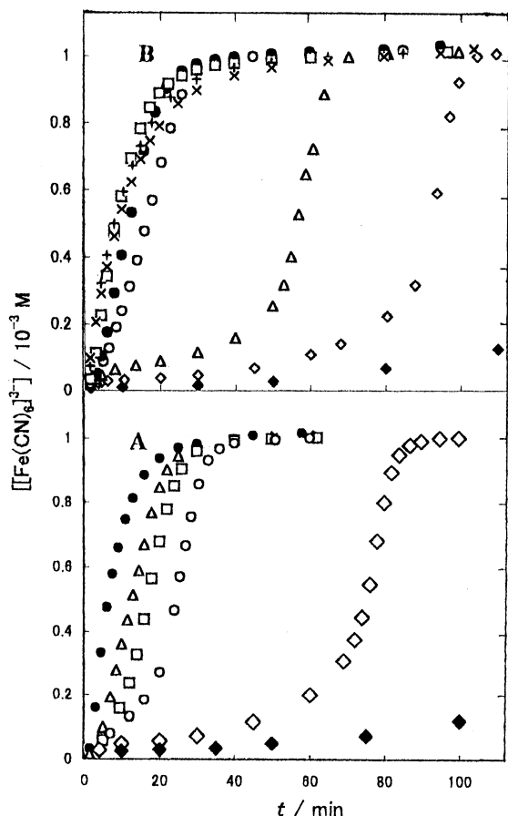
Fig. 4. Plots of [\text{Fe}(\text{CN})_6]^{3-} vs t .
